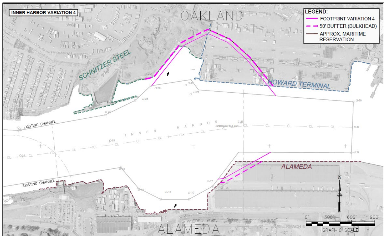
Figure 31: Inner Harbor Variation 4 - Non-Circular
