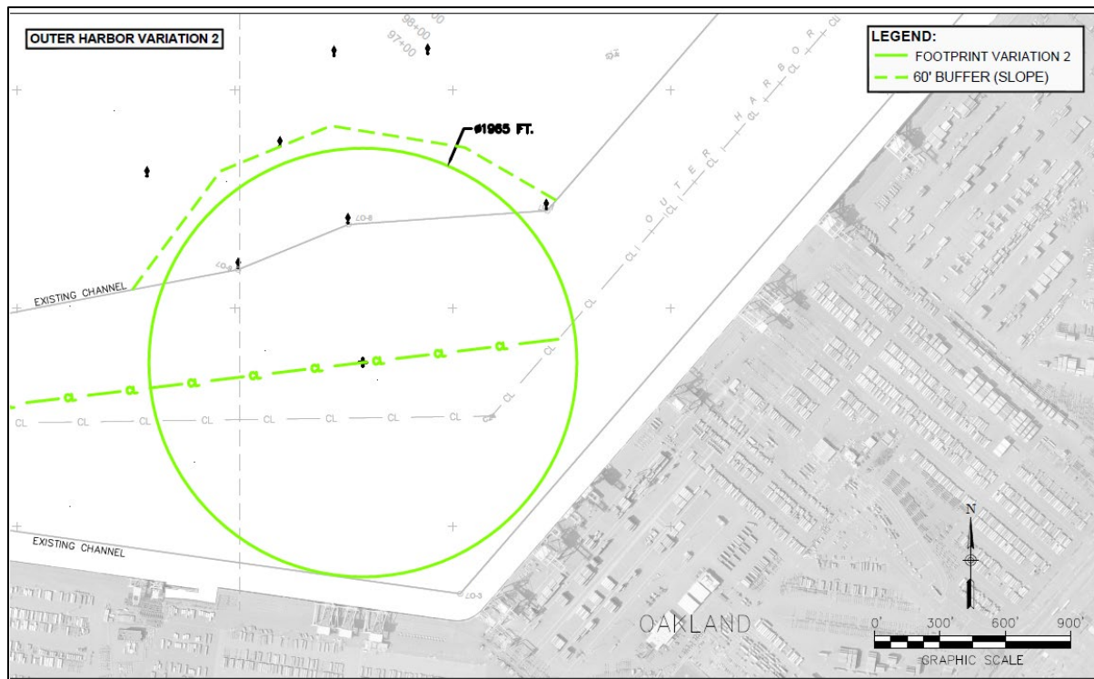
Figure 35: Outer Harbor Variation 8 - Centered
