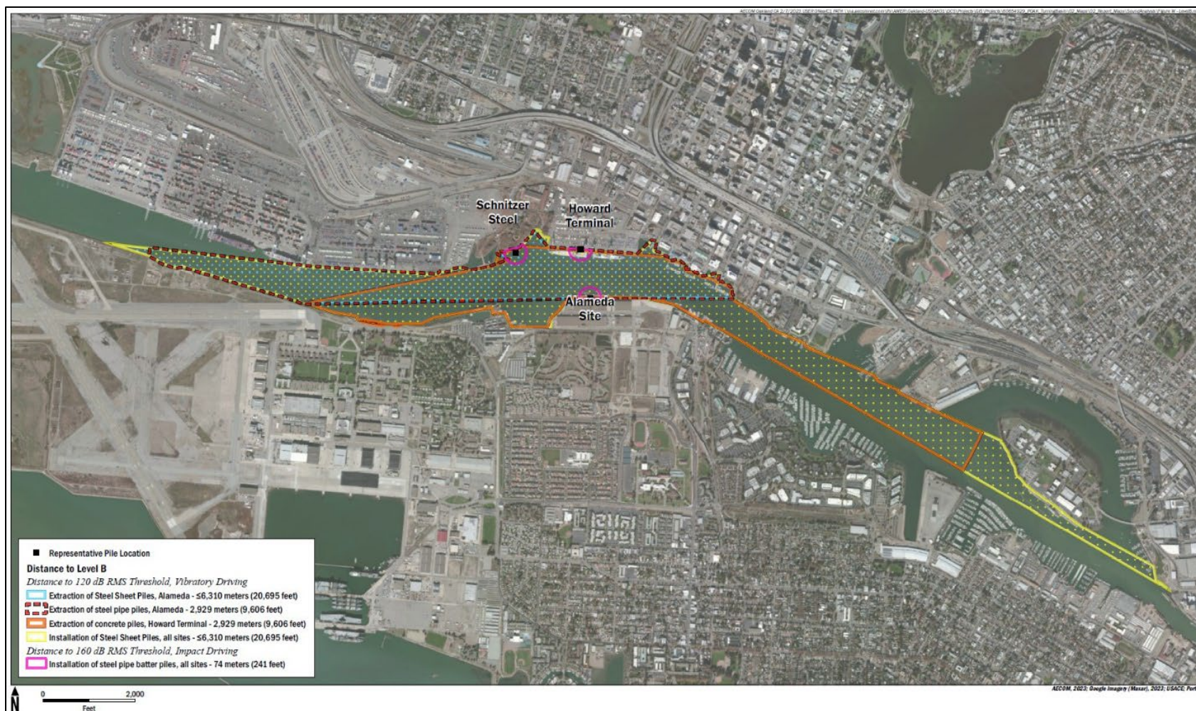
Figure 42: Distance to Level B Threshold for Marine Mammals
