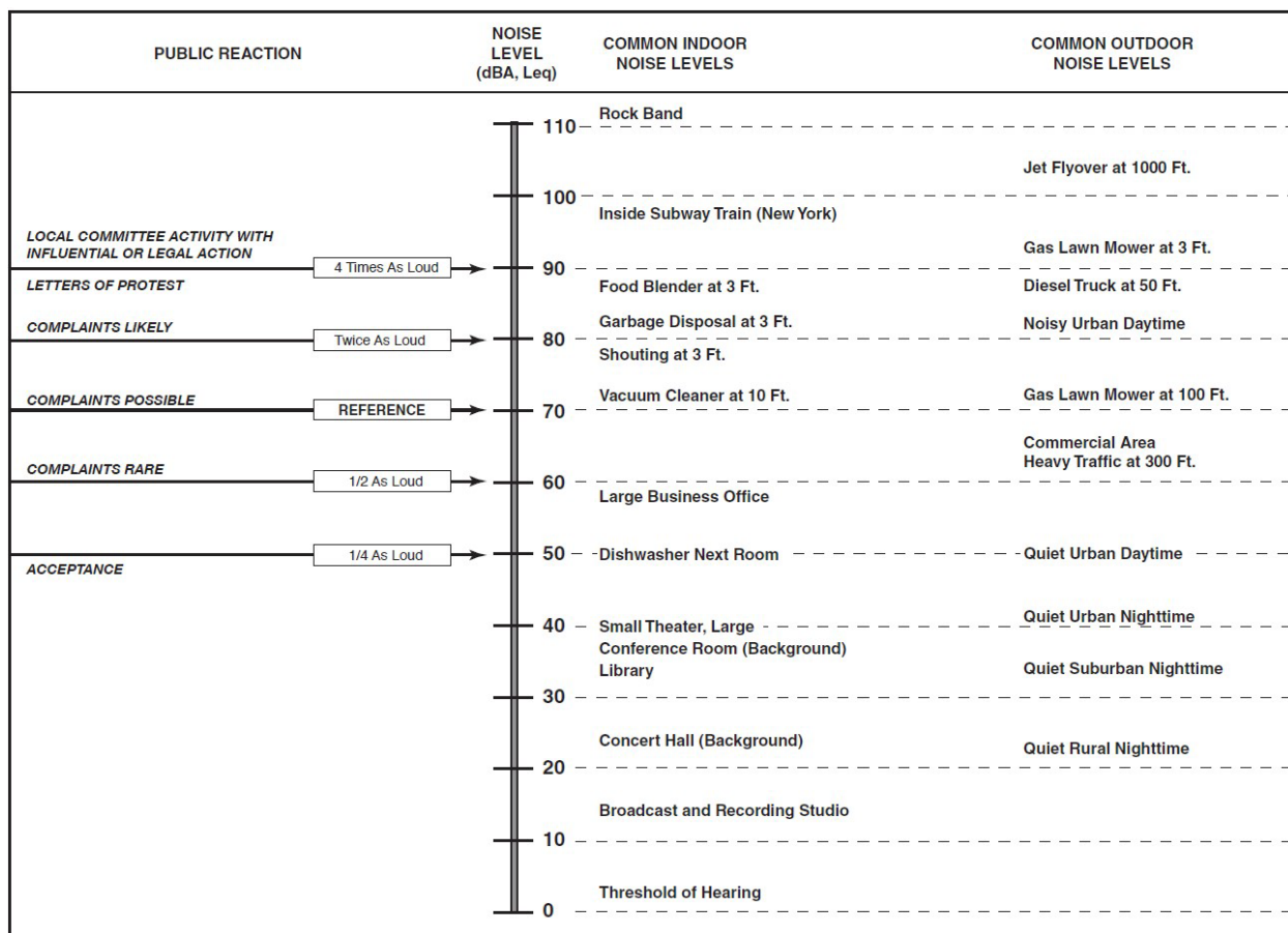
Figure 47: Effects of Noise on People
