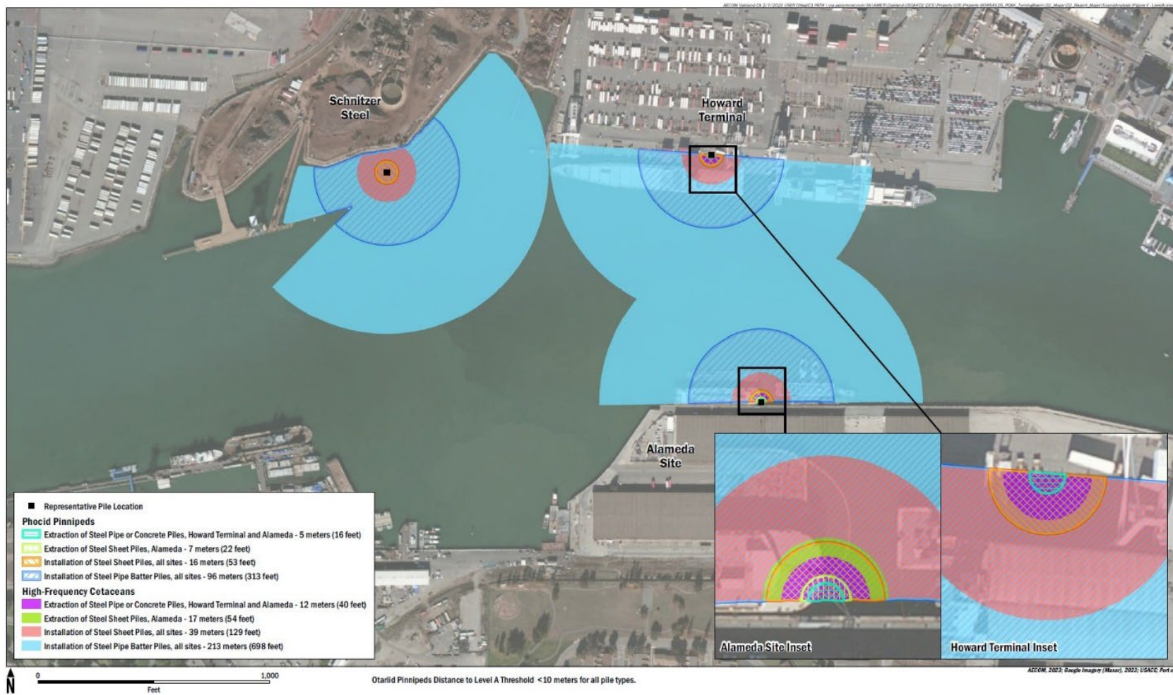
Figure 41: Distance to Level A Threshold for Marine Mammals
